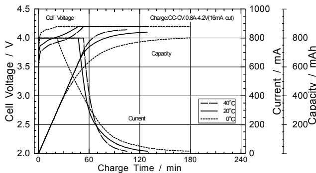
Charge characteristics
